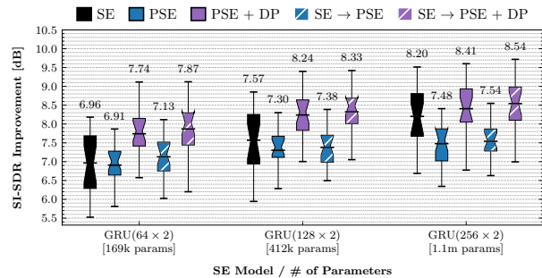
Figure 3: Box plot of experiment results with notches showing the 95% confidence interval. We report mean SI-SDR improvement over unseen mixtures across each test-time user. Model configurations are detailed in Sec. 3.1.
